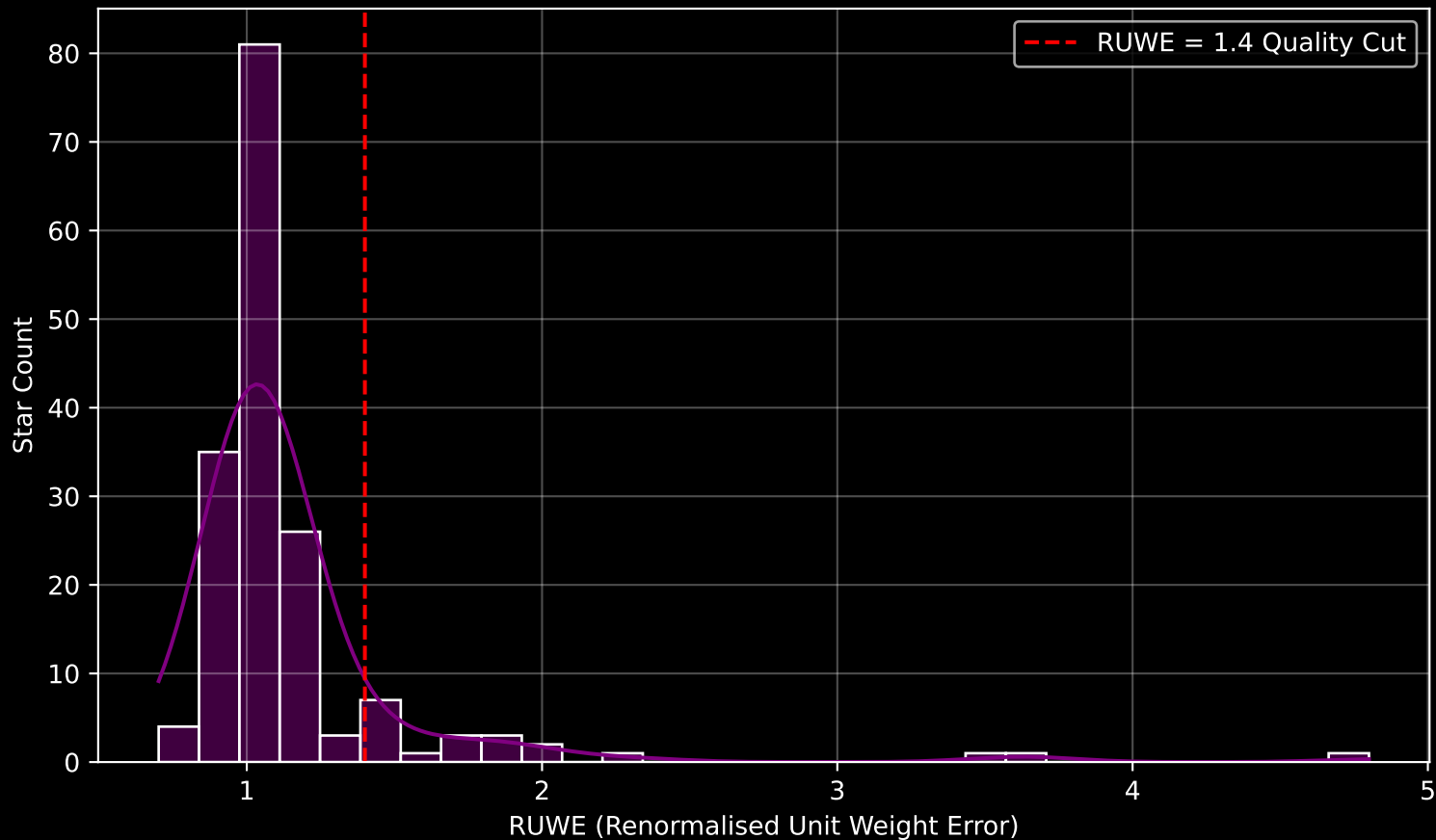
GAPOGEE DR17 Field [195+18] RUWE Distribution (n= 169)
